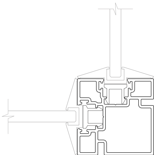
Nodo 2 vie / 2 ways joint
