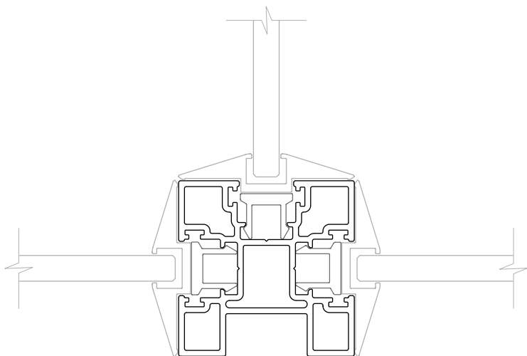
Nodo 3 vie / 3 ways joint
